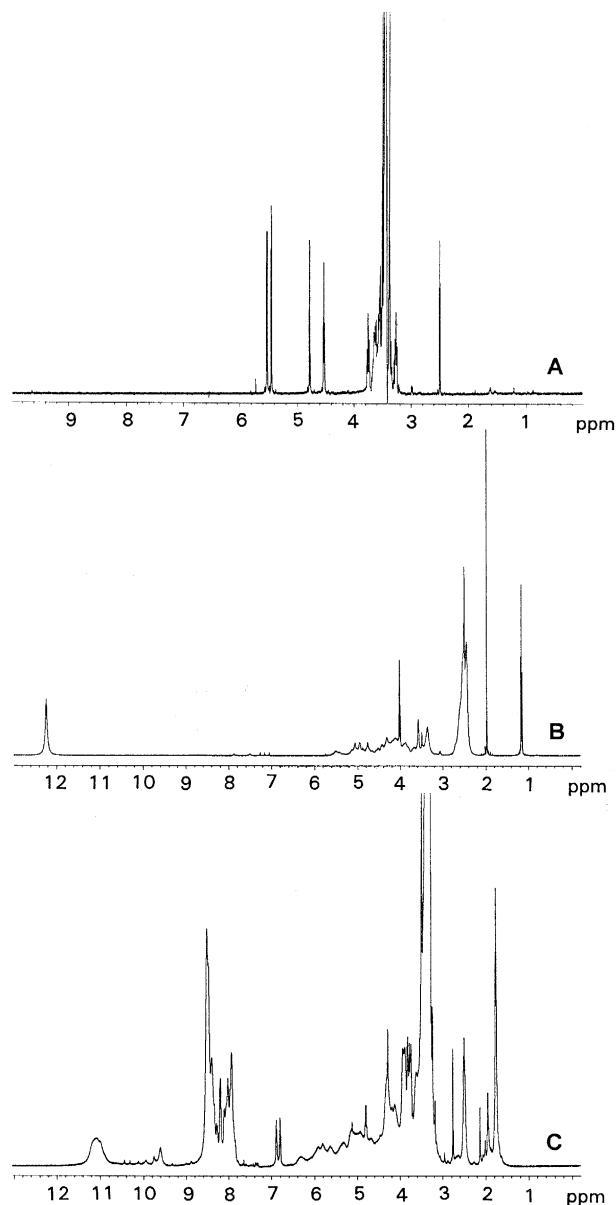
Fig. 3. ^1H -NMR spectra. (A) \alpha -Cyclodextrin. (B) Persuccinylated \alpha -cyclodextrin. (C) \alpha -Cyclodextrin conjugated to LY237868. Each compound was dissolved in DMSO-d_6 and ^1H -NMR spectra were recorded at 500 MHz.
